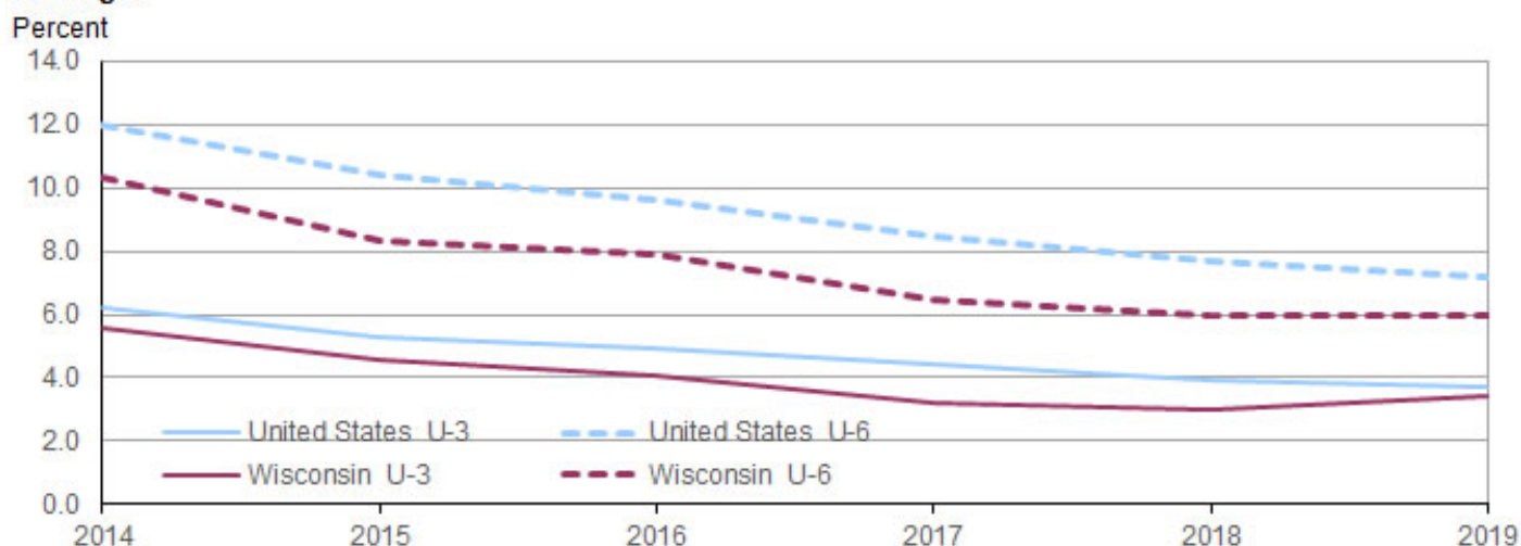
Chart 1. Two alternative measures of labor underutilization, United States and Wisconsin, 2014–19 annual averages
