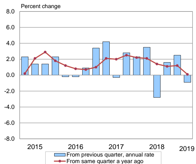
Chart 2. Unit labor costs, nonfarm business, 2015Q1 – 2019Q1
